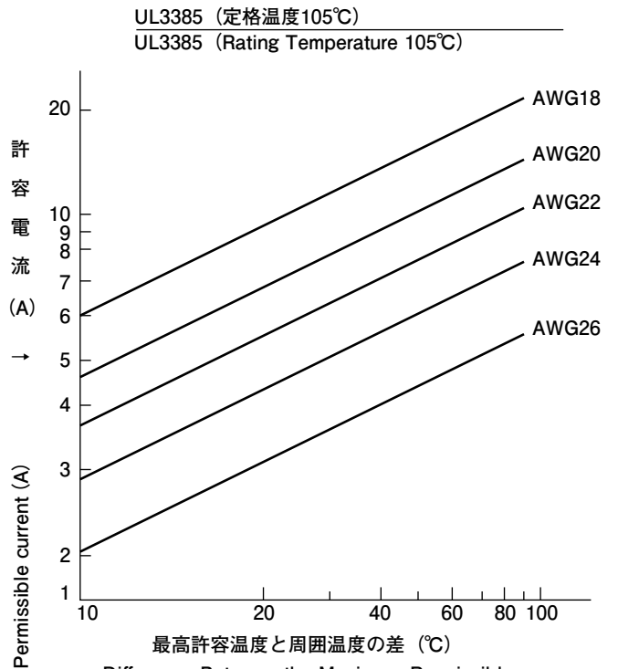
最高許容温度と周囲温度の差 (°C) Difference Between the Maximum Permissible Temperature and the Ambient Temperature (°C)
